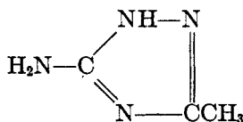
Aminomethyltriazole
