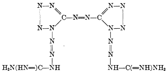
Bis-1,1(3-guanyltriazeno)-5,5-azotetrazole
